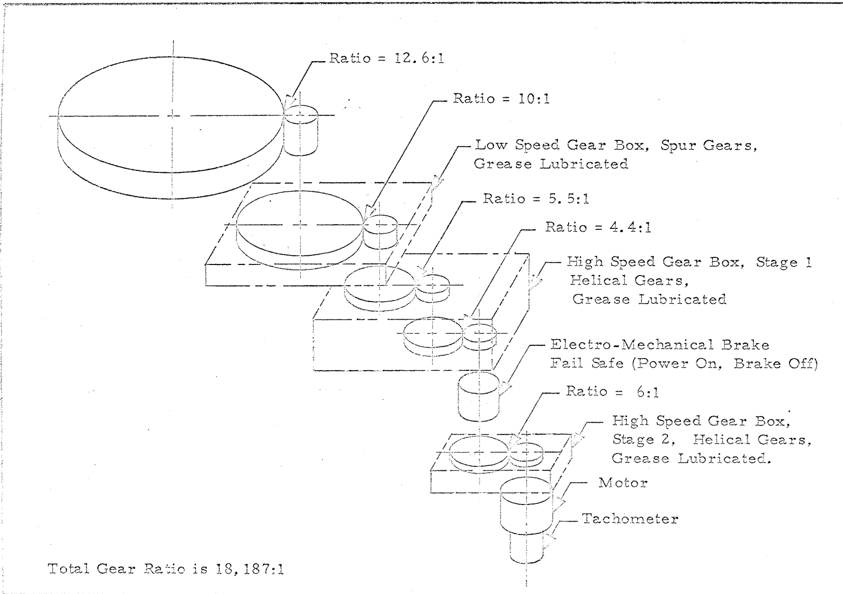
Figure 3-40 Typical Synergized El-Az Drive Train
