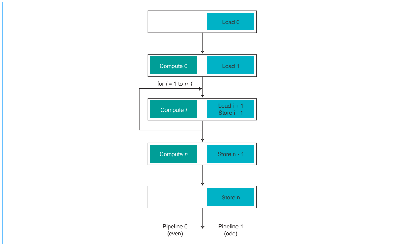
Figure 24-7. Software-Pipelined Loop
