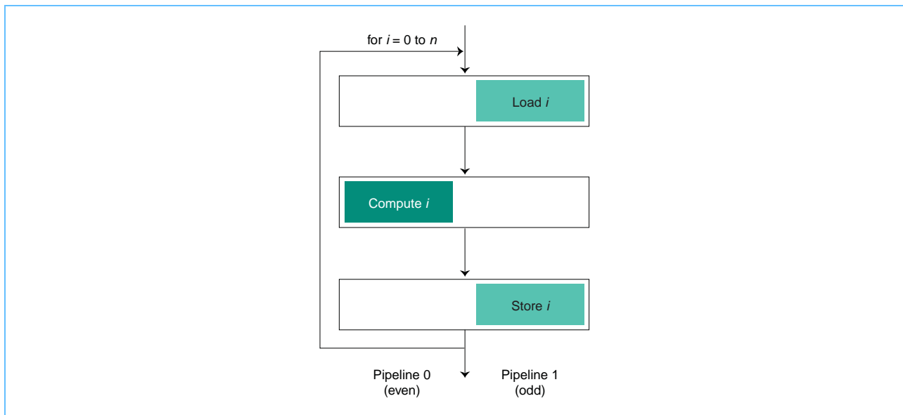
Figure 24-6. Basic Loop
