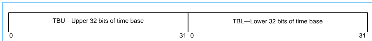
Figure 13-1. Time Base (TB) Register
