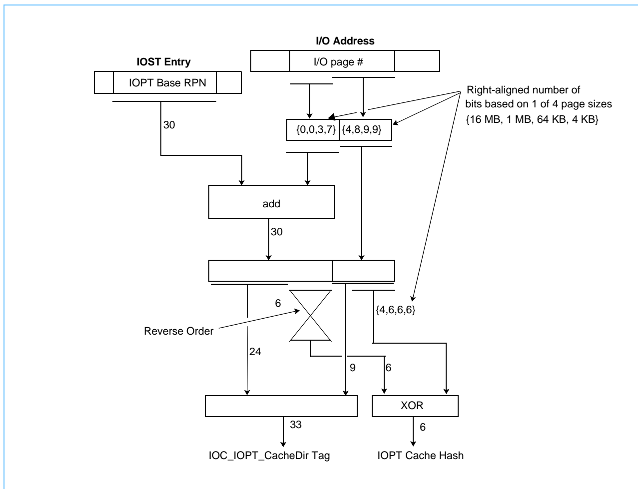
Figure 7-7. IOPT Cache Hash and IOPT Cache Directory Tag
