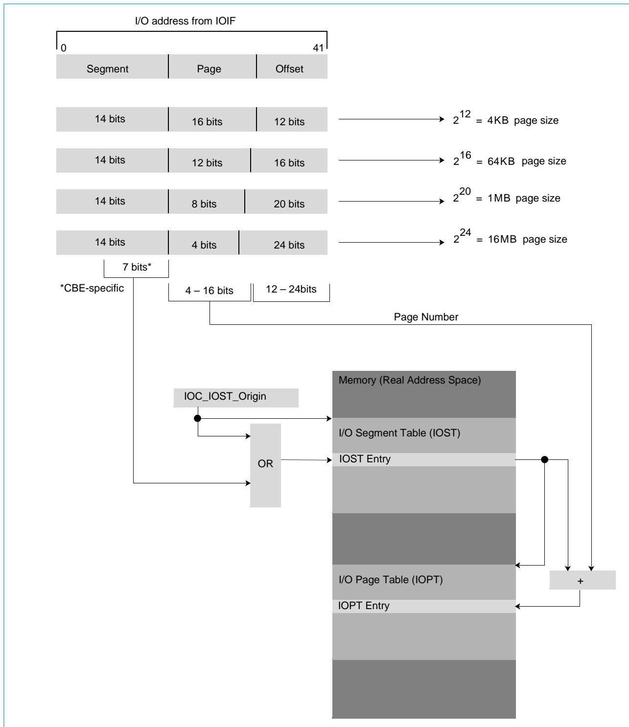
Figure 7-5. I/O-Address Translation Overview
