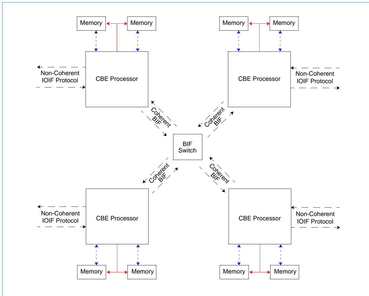
Figure 7-3. Quad CBE System Configuration
