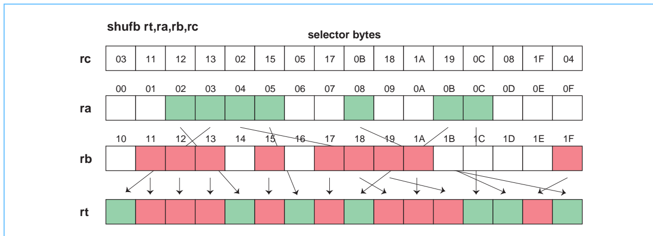
Figure 24-8. Shuffle Bytes Instruction
