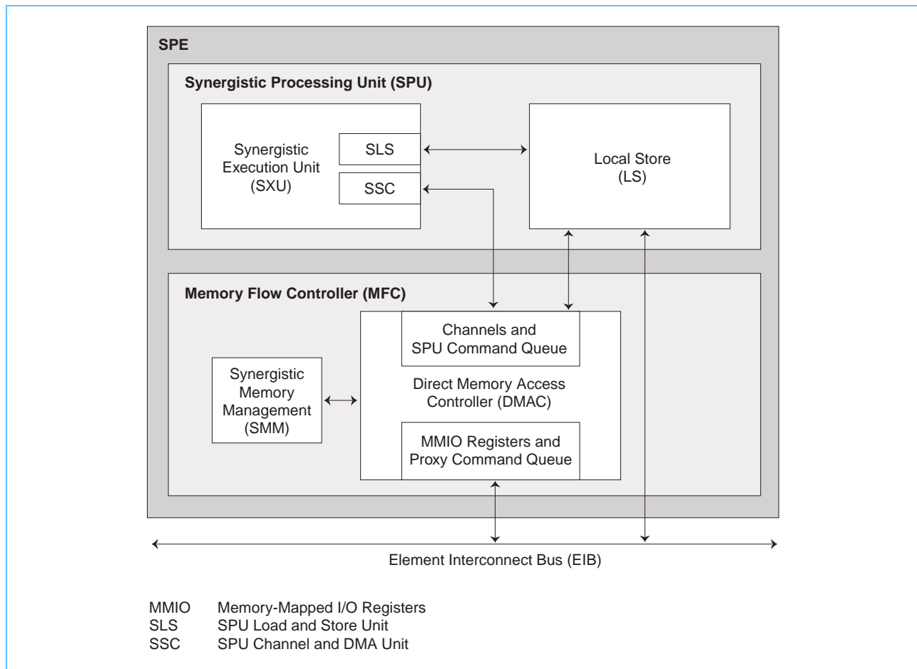
Figure 3-5. MFC Block Diagram
