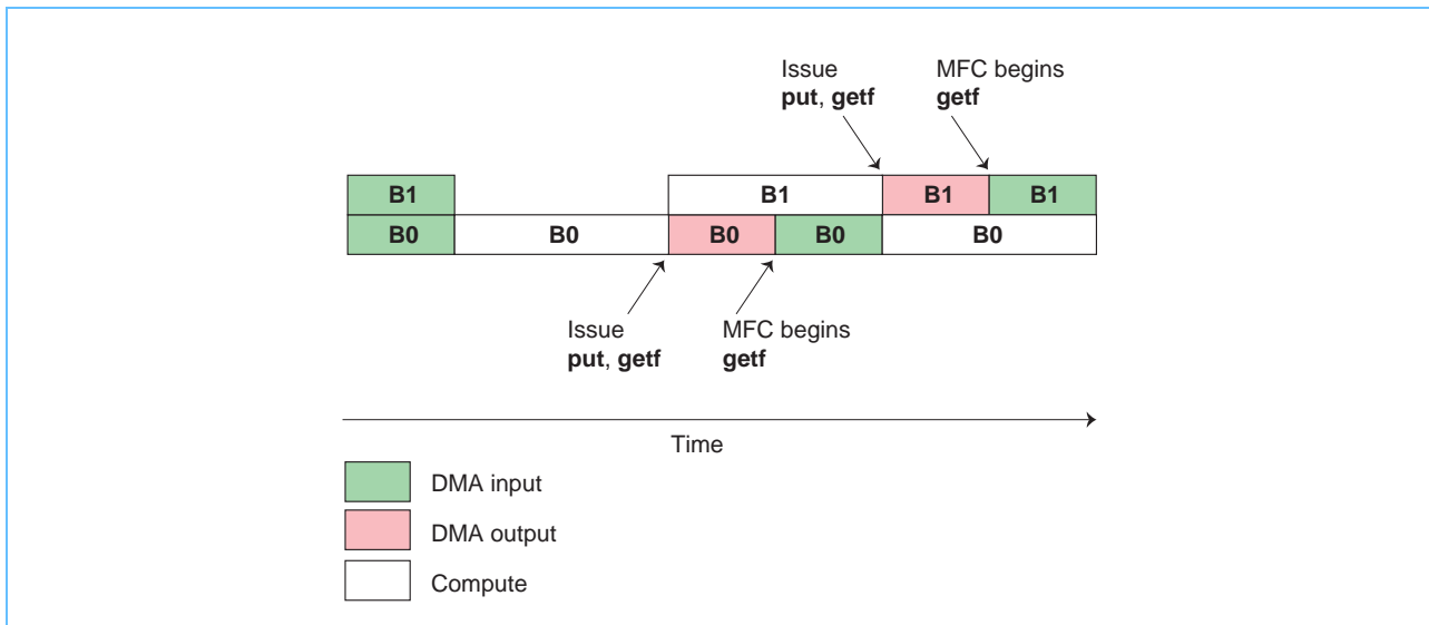
Figure 24-4. Shared I/O Buffers with Fenced get Command
