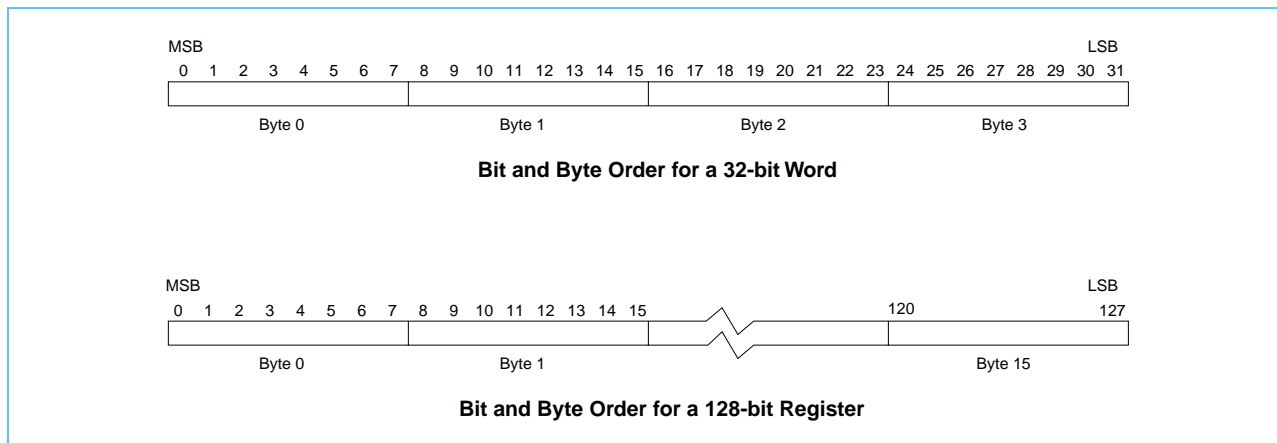
Figure 1-3. Big-Endian Byte and Bit Ordering
