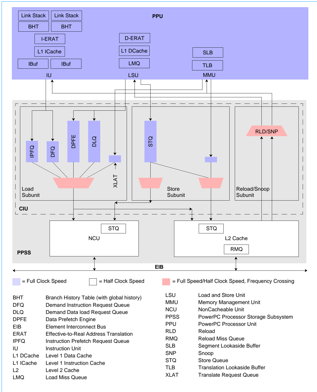
Figure 6-1. PPE Cache
