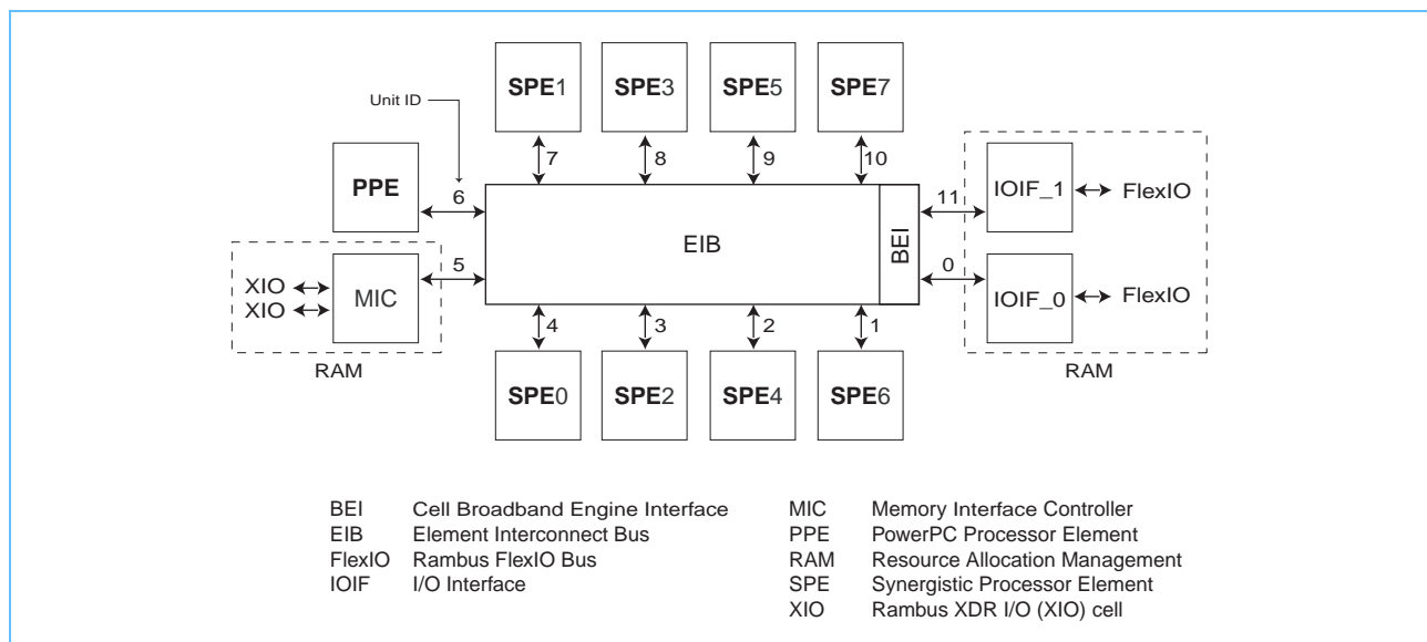
Figure 1-1. Cell Broadband Engine Overview
