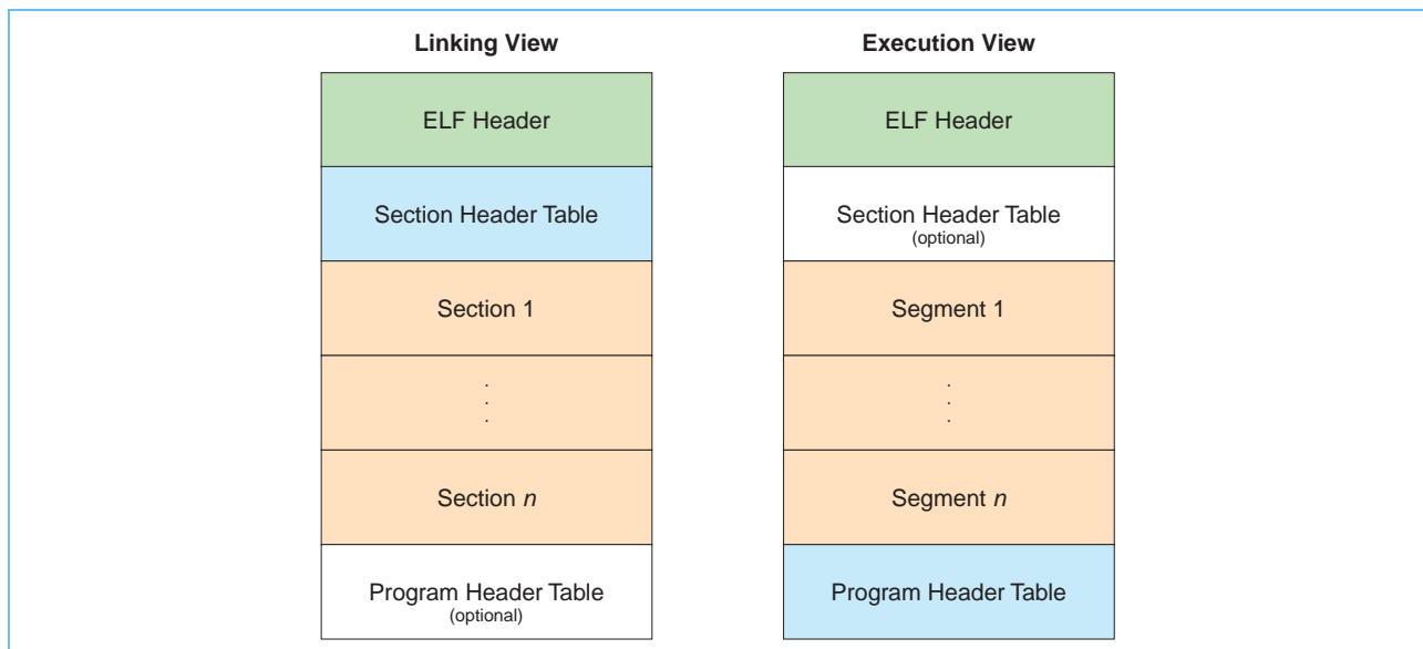
Figure 14-1. Object-File Format
