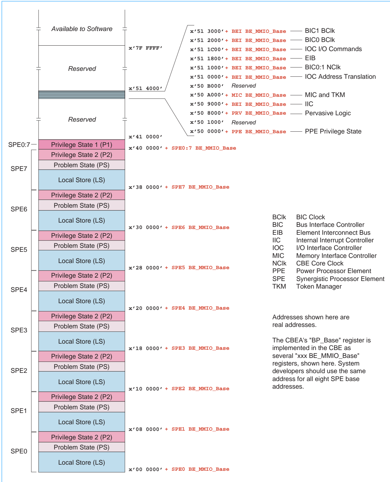
Figure 5-1. CBE Memory Map
