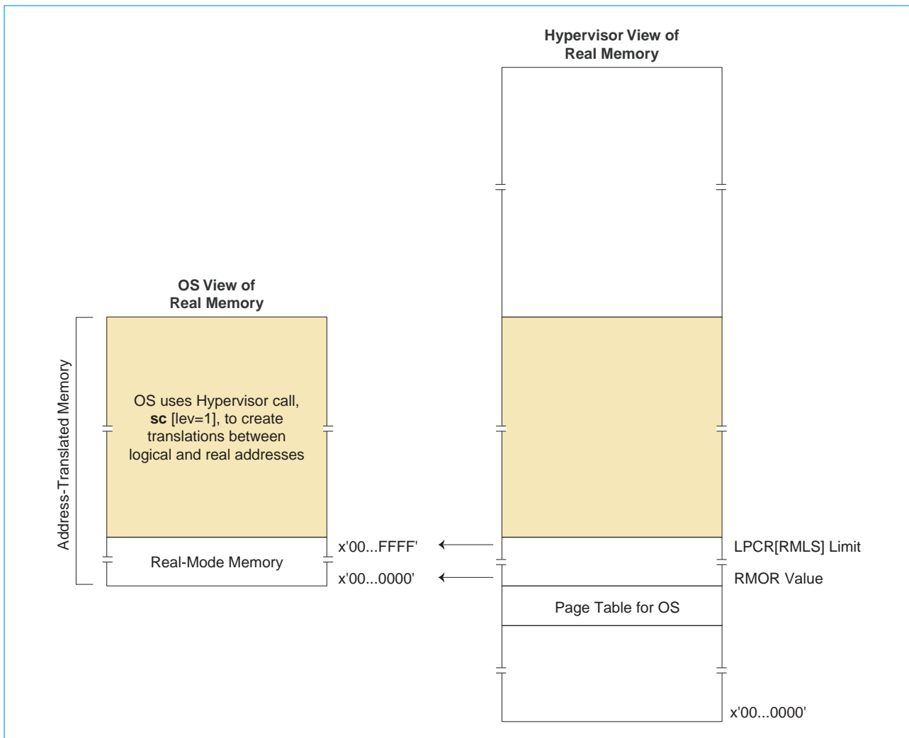
Figure 11-3. Operating-System and Hypervisor Views of Physical Memory
