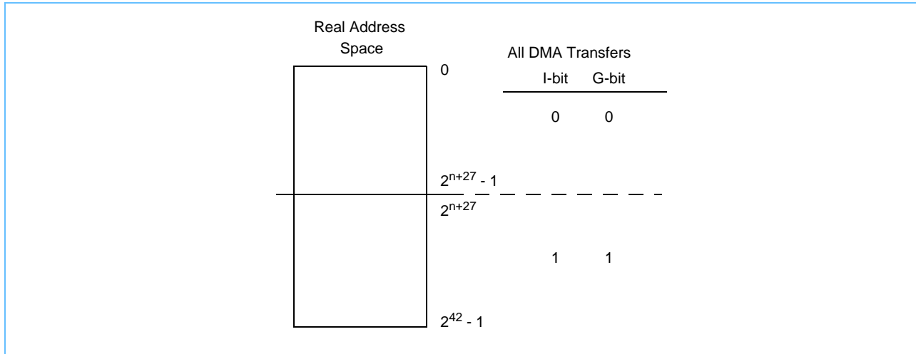
Figure 4-9. Real-Mode Storage Boundary
