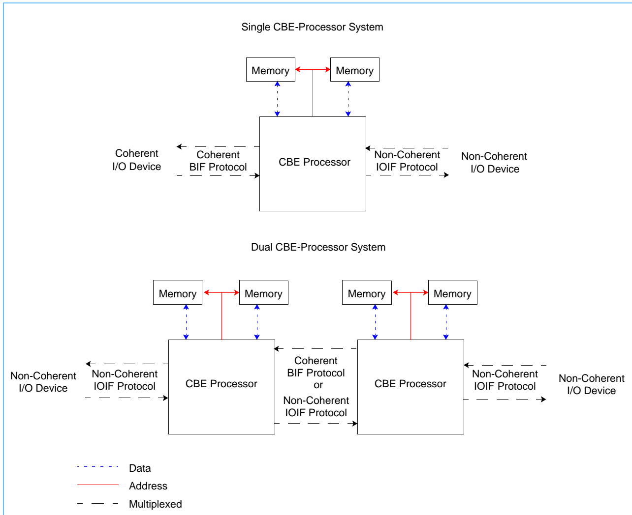
Figure 7-2. Single and Dual CBE System Configurations
