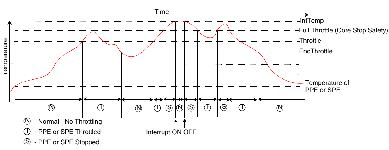
Figure 15-1. Digital Thermal-Sensor Throttling
